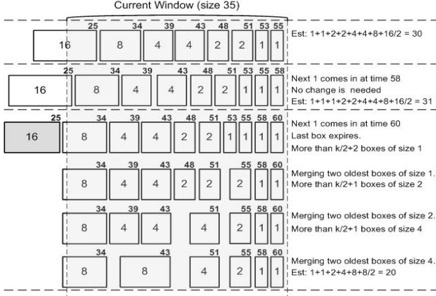
Figure 1: Incrementing an EH sketch twice at time 58 and 60. That is we have seen 1, 0, and 1 respectively at time 58, 59, and 60. ( k=2 and W=35 )
