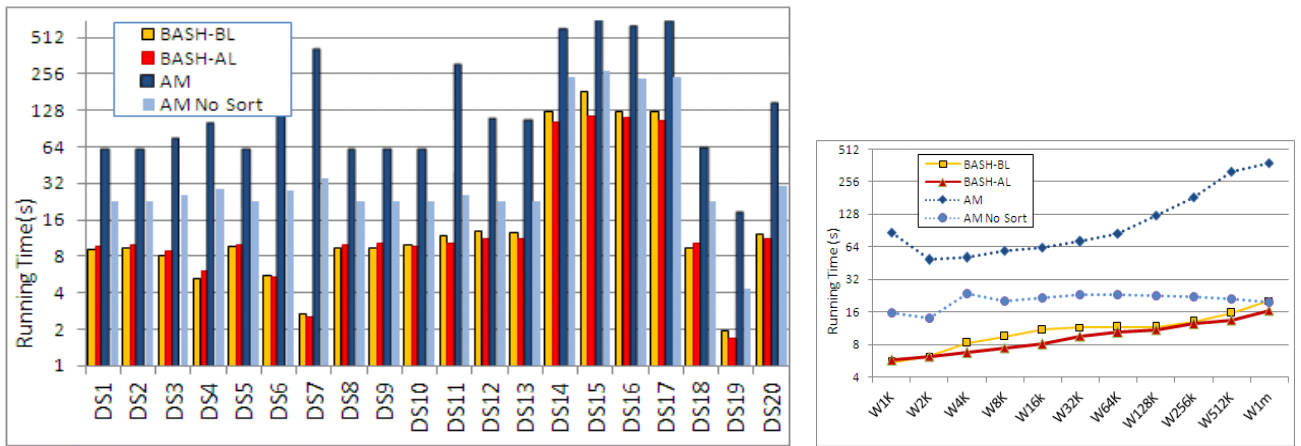
Figure 3: a) Execution time for all data sets ( W = 100k ), and b) The effect of changing window size from 1k to 1m on the execution time on DS13. ( k = 10 , p = 7 , and \epsilon = 0.01 .)
