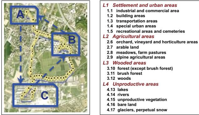
Figure 3: Region Annotation
