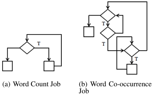
Figure 5: CFGs of the Map Functions of the Word Count and Word Co-occurrence MR Jobs
