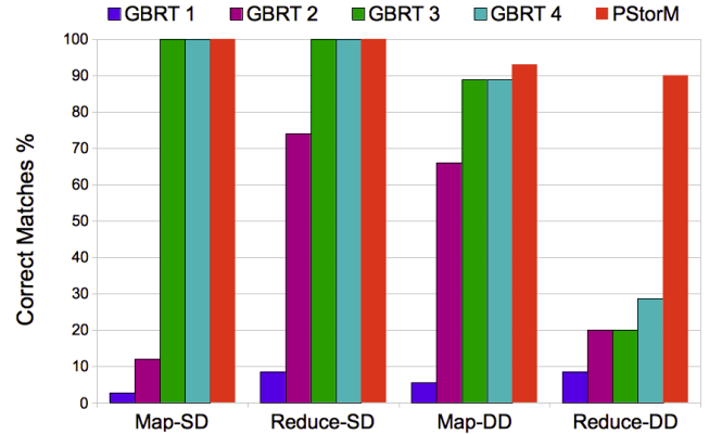
Figure 8: Correct Match Percentages for the Alternative Matching Solution (GBRT) with Different Parameter Settings vs. PStorM in the Two Content States of the Profile Store (SD and DD)
