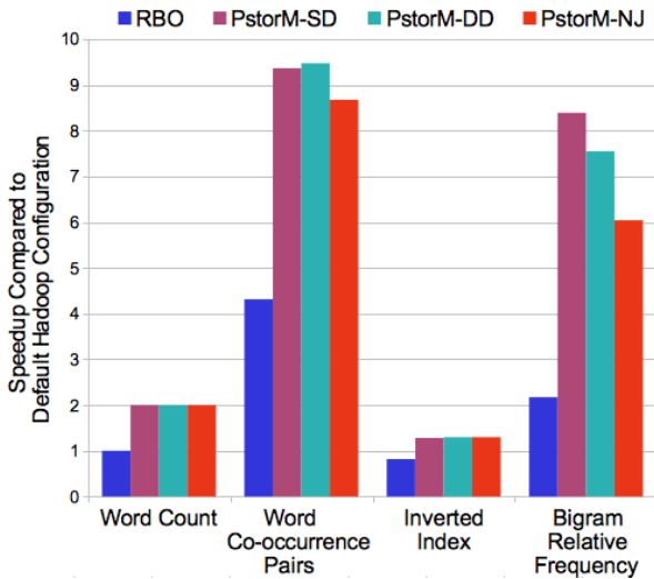
Figure 9: Speedups of Different MR Jobs Executed with the RBO Recommendations and the CBO Recommendations Based on a Profile Returned by PStorM at the Three Content States of the Profile Store (SD, DD, and NJ)
