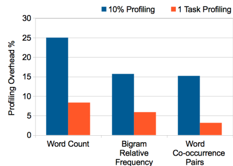
Figure 4: Profiling Overhead for 10% Profiling and 1 Task Profiling as a Fraction of the Job Runtime using the RBO Recommendations Without Profiling
