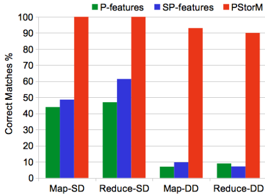
Figure 7: Correct Match Percentages for the Two Alternative Feature Selection Solutions (P-features and SP-features) vs. PStorM in the Two Content States of the Profile Store (SD and DD)
