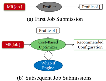
Figure 3: Starfish Tuning Workflow
