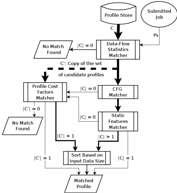
Figure 6: The Map/Reduce Profile Matching Workflow
