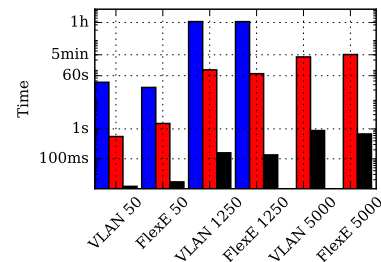
Figure 8: Average computation times of each algorithm.
